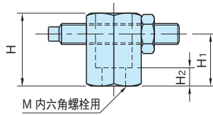
BJ210-S (短小型)
