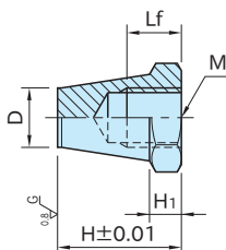
BJ810-F (前端研磨型)
