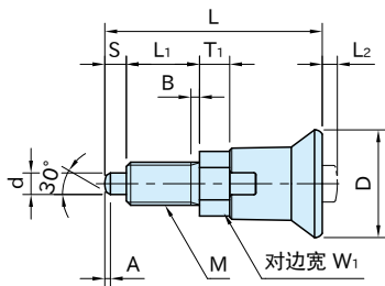
BNDXN BNDXN-A-SUS (单螺母)
