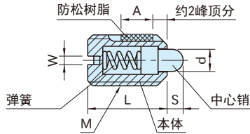
螺丝尺寸: M8~M16
