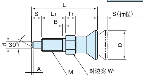
NDXNE NDXNE-SUS NDXNE-A-SUS (单螺母)
