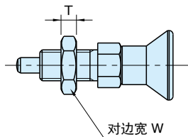
NDXNE-W NDXNE-W-SUS NDXNE-AW-SUS (双螺母)
