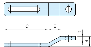
CRT (曲柄型张紧器)
